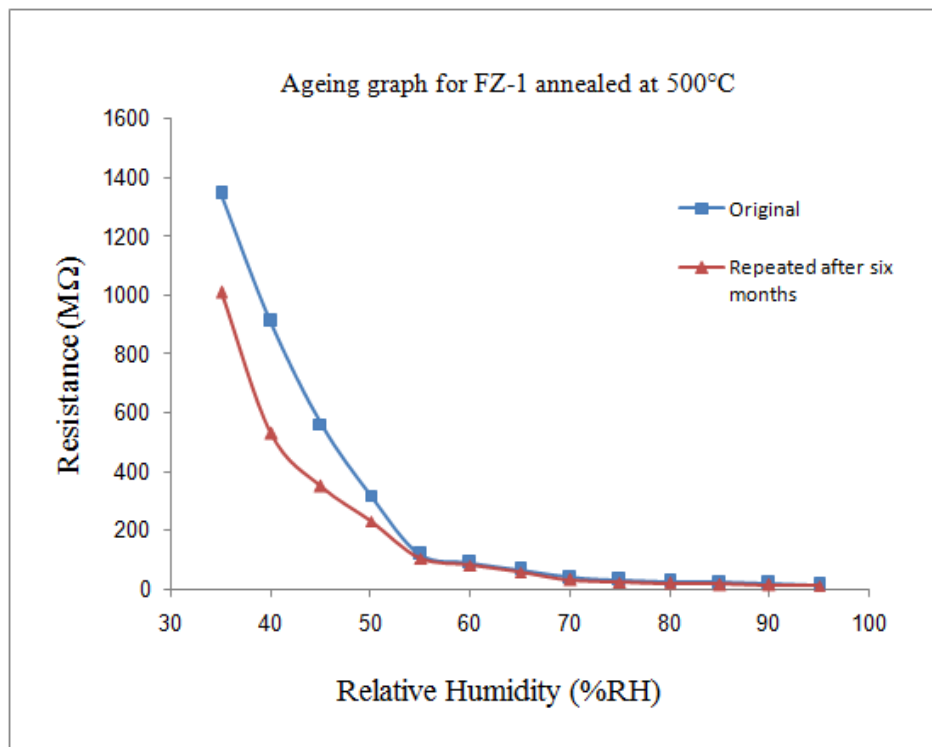
Fig.3. Aging effect behavior of sample FZ-1 annealed at 500°C.
